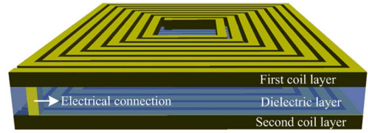
Fig. 5. Configuration of a dual-layer inductor.
