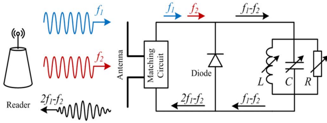
Fig. 7. The operation principle of the intermodulation sensor system.
